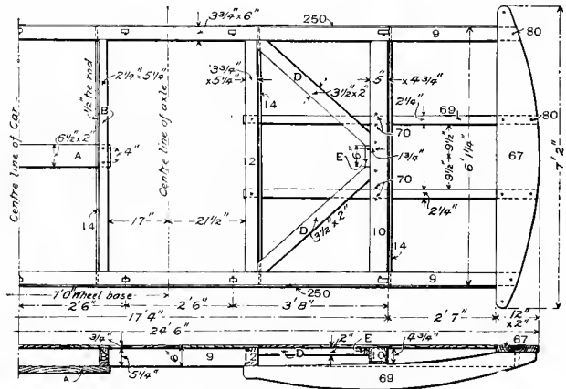
Fig. 5660. Half Plan.
